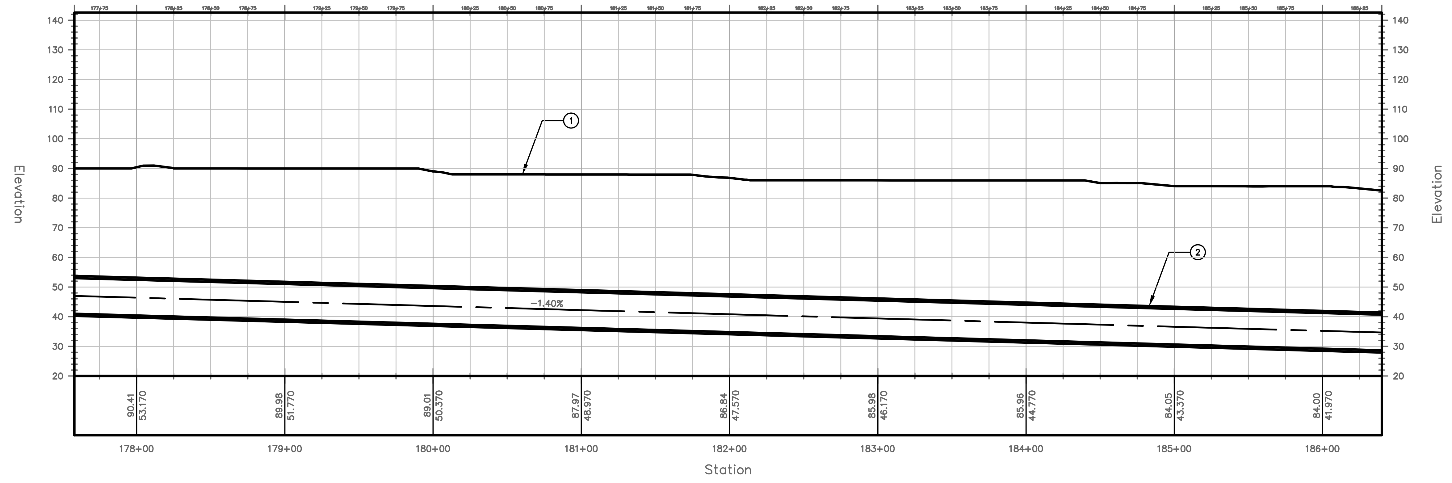
PROFILE VIEW HORIZONTAL SCALE: 1"=40' VERTICAL SCALE: 1"=20'
