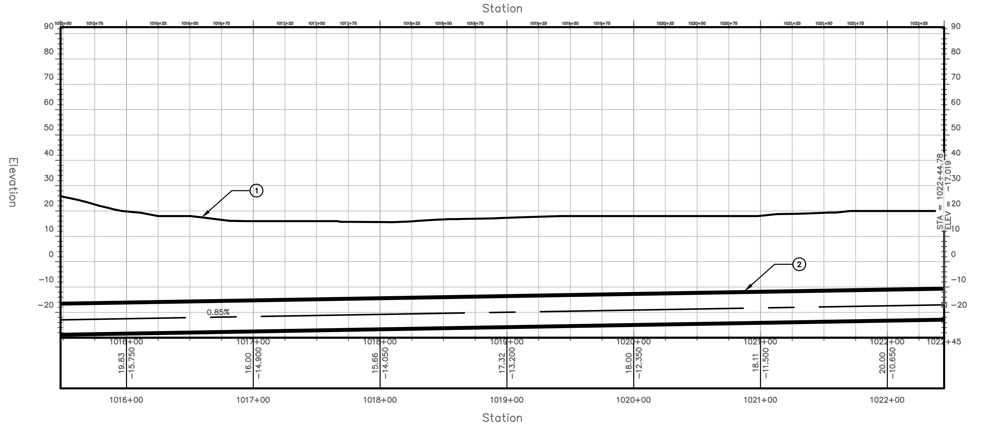
PROFILE VIEW HORIZONTAL SCALE: 1"=40' VERTICAL SCALE: 1"=20'
